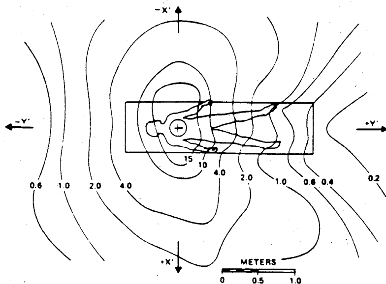
FIGURE 2. Pattern in the horizontal plane of exposure value (milliroentgen/hour) during cardiac catheterization. Typical values of 96 kVp, 10 X 10 cm field and 1.95 R/min tabletop exposure rates were used. (Reprinted by permission of the American Heart Association and from Rueter. 6 )
